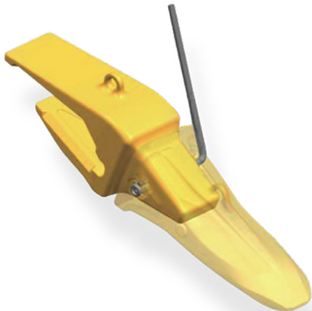
G.E.T. SYSTEM New Hammerless Version (Available for all RC Teeth)
